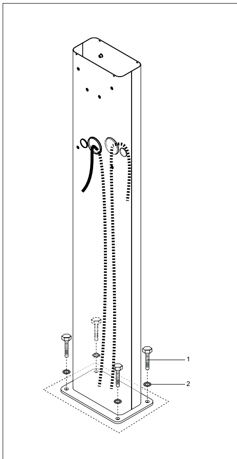
Fig. 03: Final mounting
