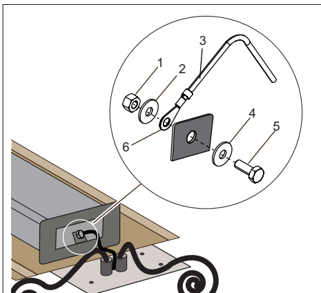
Fig. 01: Ground connection
